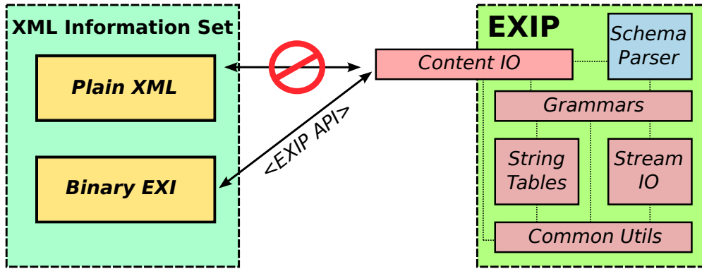
Figure 2.1: EXIP components
